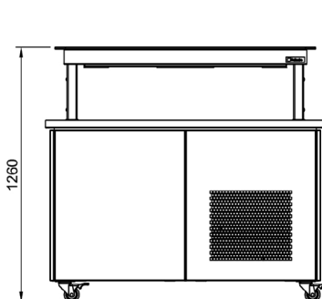
Front Elevation
